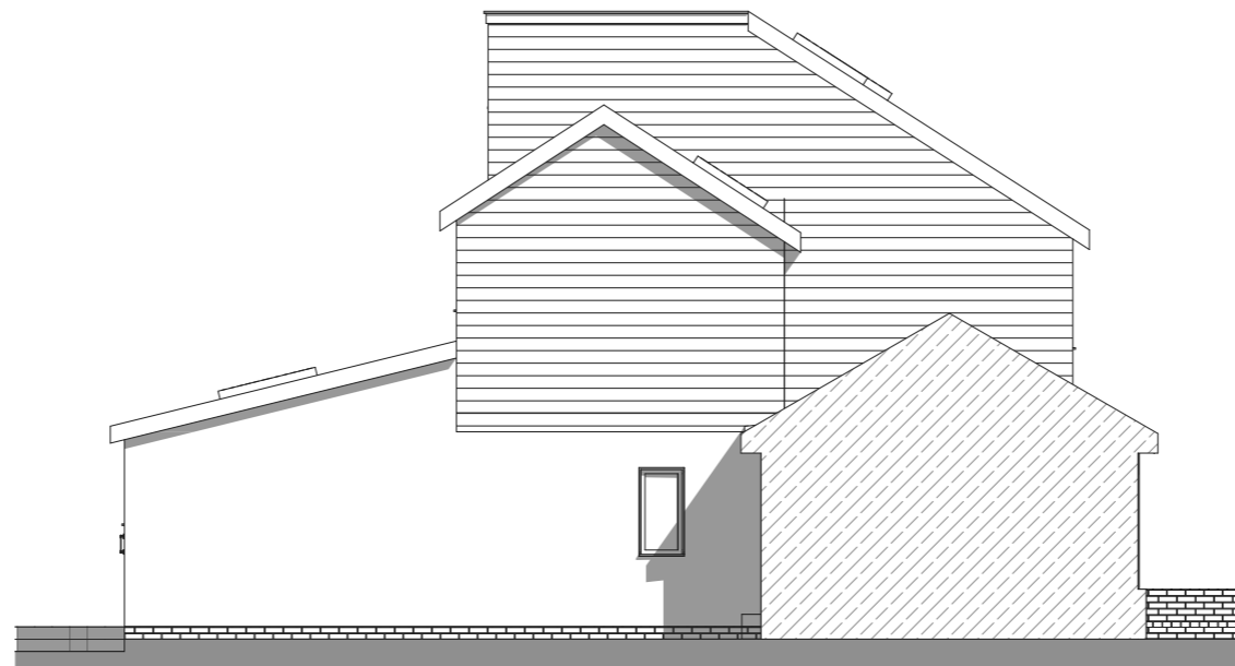
2 SIDE ELEVATION 1:100
